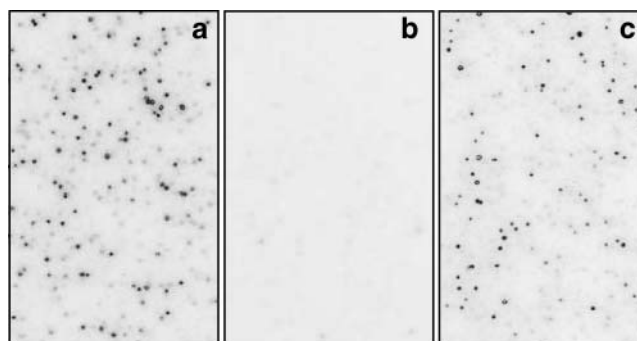
FIGURE 4 Encapsulated hairpin ribozyme molecules are protected against ribonuclease digestion. Each panel shows an image of a surface on which fluorescent hairpin ribozyme molecules are attached, either directly or encapsulated. (a) Ribozyme molecules directly immobilized on the surface before treatment with ribonuclease (RNaseA). (b) Ribozyme molecules directly immobilized on the surface after treatment with ribonuclease. The absence of fluorescence indicates that the ribozymes have been digested by the enzyme, allowing free diffusion of the fluorophores away from the surface. (c) Encapsulated ribozymes following treatment with ribonuclease. Unlike b , the encapsulated molecules are clearly not accessible to the enzyme, and thus the surface-bound fluorescence is preserved.
