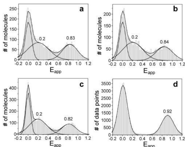
FIGURE 6 Variation of FRET efficiency with respect to the extravesicular conditions for encapsulated hairpin ribozymes. Histograms of the number of observed molecules displaying a given apparent FRET efficiency for encapsulated ribozymes in the presence of (a) 0.5 mM Mg^{2+} ; (b) 0 mM Mg^{2+} , 1 mM EDTA; (c) 1 mM Mg^{2+} ; (d) 0.5 mM Mg^{2+} , 1 M NaCl. For the conditions a–c, the differences in the extra- and intravesicular conditions did not induce significant size changes for the vesicles and the ribozymes were not affected by the various extravesicular Mg^{2+} concentrations. The FRET histograms reveal the same dynamic behavior, i.e., the molecules fluctuate between folded ( E_{app} \sim 0.9 ) and unfolded ( E_{app} \sim 0.25 ) states. In d, 1 M NaCl caused osmotic shrinking of the vesicles and a consequent increased concentration of Mg^{2+} inside the vesicle. All ribozymes adopt the folded conformation as a result, with the loss of the peak corresponding to E_{app} \sim 0.25 .
